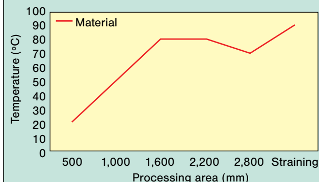
Figure 6 - temperature profile along the rolls
