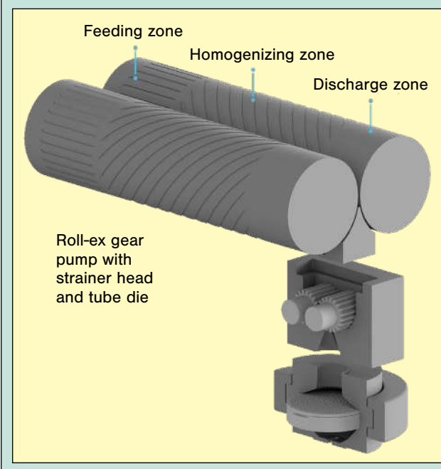
Figure 3 - basic principle of TRP technology
