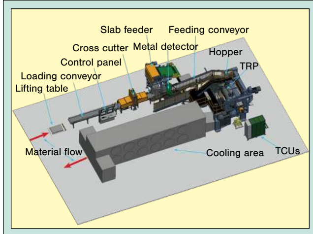
Figure 5 - complete solution: TRP reworker
