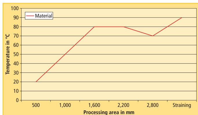
Fig. 5: Temperature profile along the rolls
