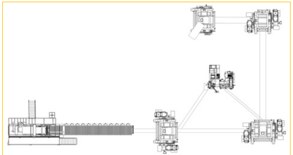
Fig. 2: Open-mill line
