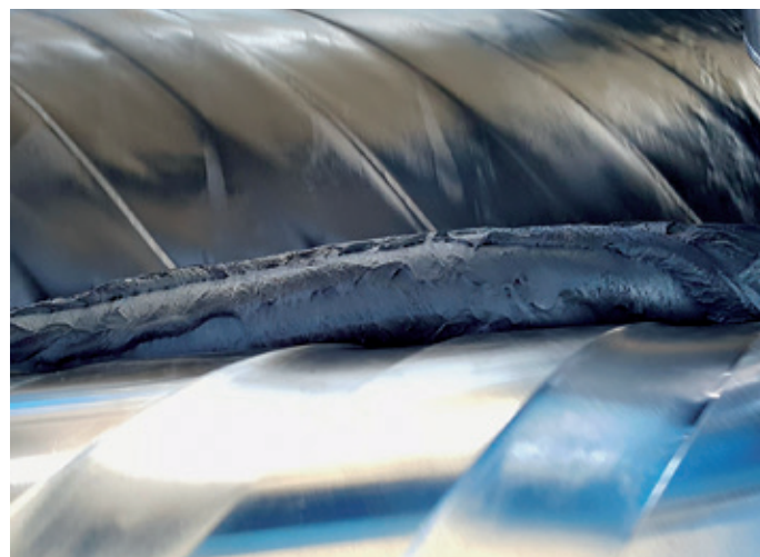
Fig. 4: Homogenisation of the compound on the nip of the open-mill
