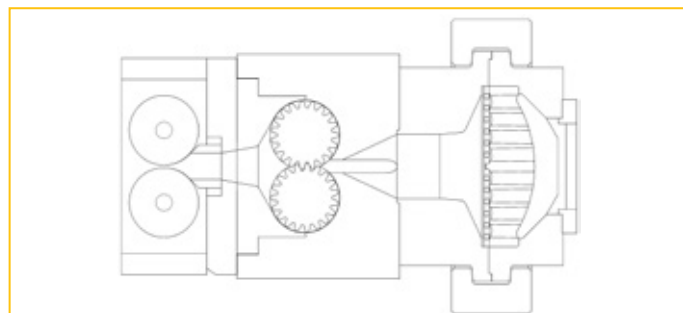
Fig. 7: Gear pump extruder with two-roll feeder
