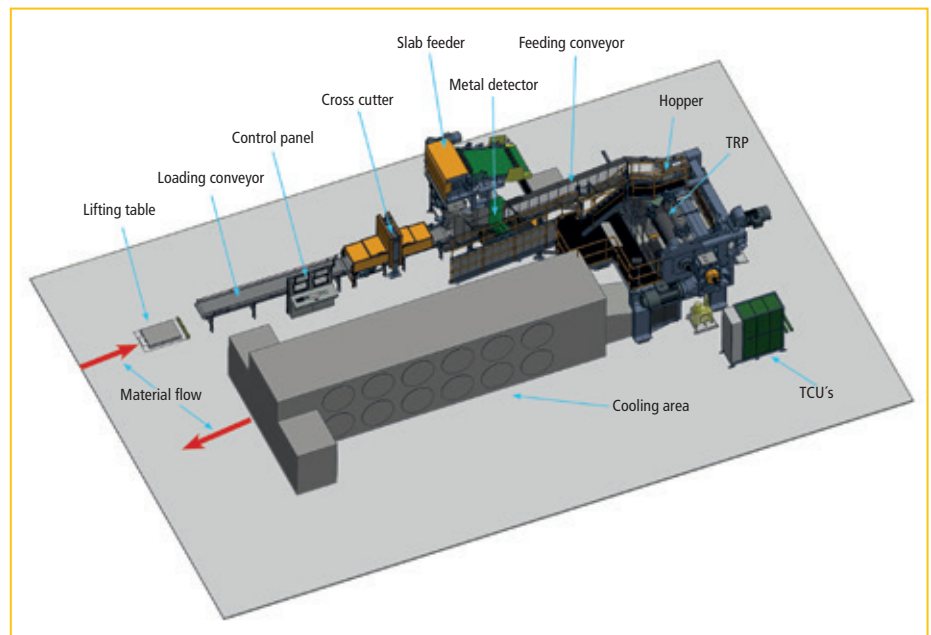
Fig. 6: The complete solution – TRP Reworker
